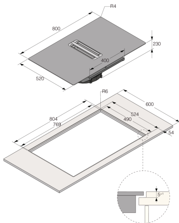
Flush installation
