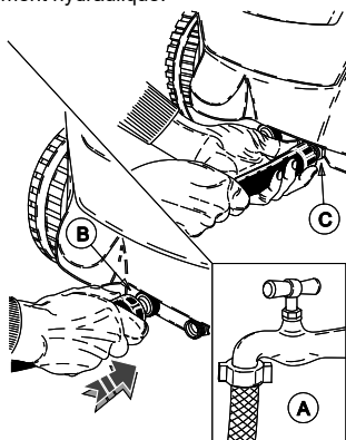
Raccordement hydraulique.
